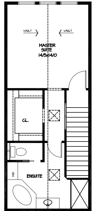
○ CRAFTSBURY II UPPER FLOOR AREA = 534 S.F.
