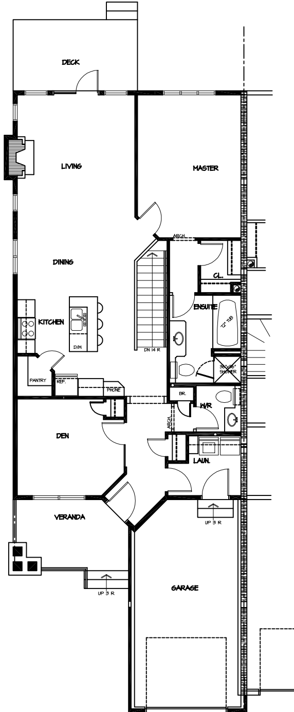
○ BENNINGTON MAIN FLOOR PLAN - 1215 SQ. FT.
