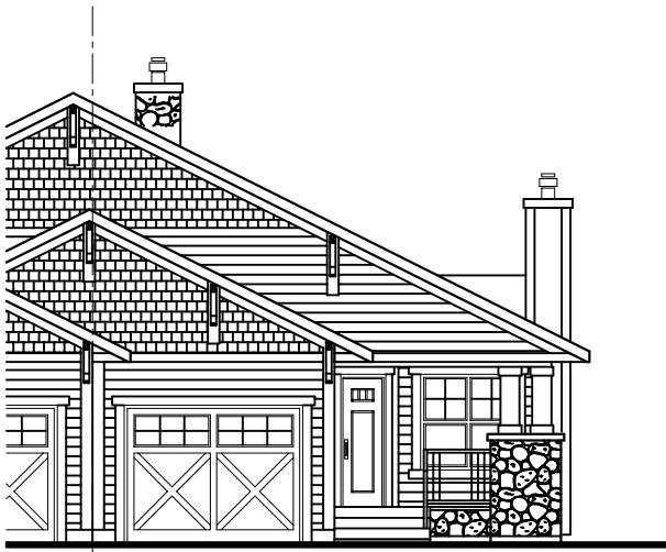
MORGAN FRONT ELEVATION
